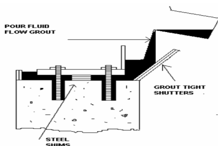
Figure 1. Grout shutter detail
